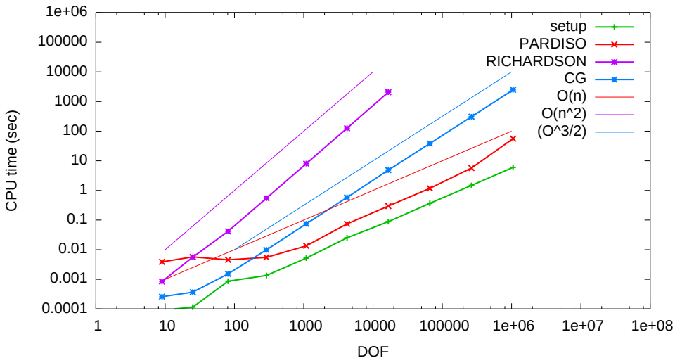
SOLVER performance for the 2D model problem
