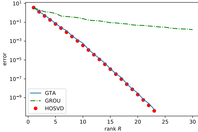
FIGURE 1. Errors in Frobenius norm for Example 1 plotted over the rank R (i.e., the number of iterations for GTA and GROU and the truncation rank for HOSVD).
