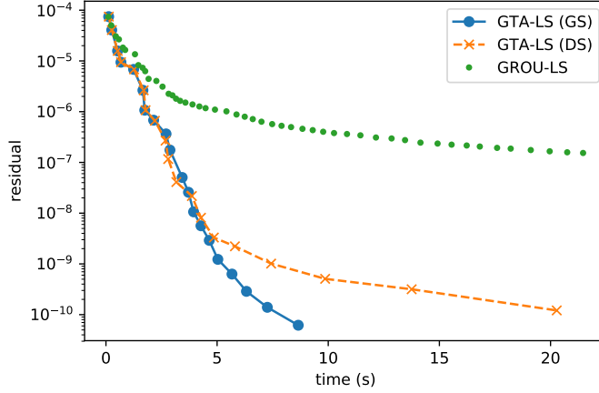
FIGURE 4. Residual norm in Example 2 (solution of Poisson equation with n = 200 ) plotted over computation time. We compare Algorithm 4.3 with direct solution of the core linear system (GTA-LS (DS)), Algorithm 4.3 with 5 Gauss-Seidel steps for the core linear system (GTA-LS (GS)), and Algorithm 4.2 (GROU-LS). Numbers are averaged over 20 runs.
