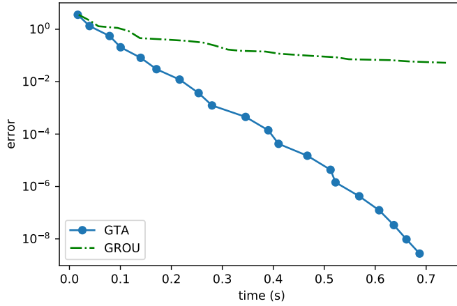
FIGURE 2. Errors in Frobenius norm for Example 1 plotted over computation time for algorithms GTA and GROU. Numbers are averaged over 25 runs.
