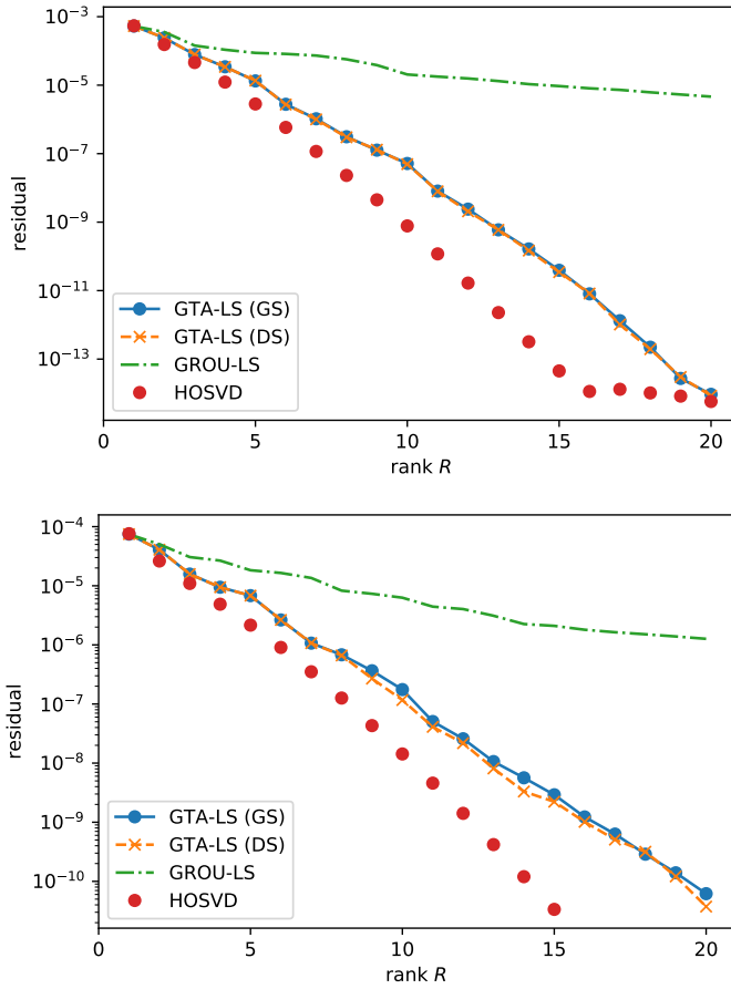
FIGURE 3. Residual norm in Example 2 (solution of Poisson equation) plotted over the rank R . Top: n = 50 , bottom: n = 200 . We compare Algorithm 4.3 with direct solution of the core linear system (GTA-LS (DS)), Algorithm 4.3 with 5 Gauss-Seidel steps for the core linear system (GTA-LS (GS)), and Algorithm 4.2 (GROU-LS). In addition, we show the residuals for the truncated HOSVD, which was computed from the full exact solution. Numbers are averaged over 20 runs.
