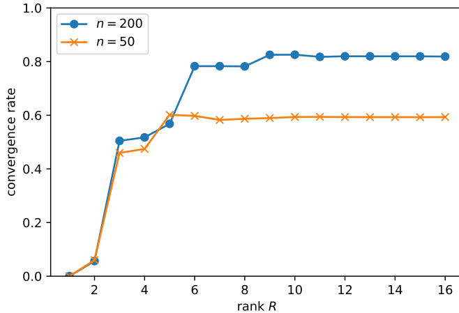
FIGURE 5. Convergence rate of Gauss-Seidel for the dense core linear system, computed as the spectral radius \rho(I - L_C^{-1}C) , for Poisson problem (Example 2) with n = 50 and n = 200 , plotted over the rank R . The size of the dense matrix C is R^3 \times R^3 .
