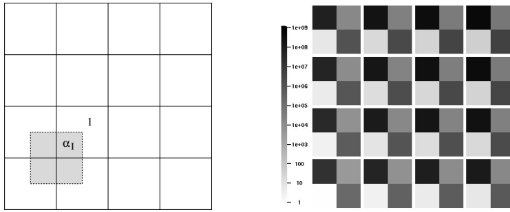
FIGURE 9. Left coefficient distribution in Example 3, right coefficient distribution and subdomain partitioning in Example 4
